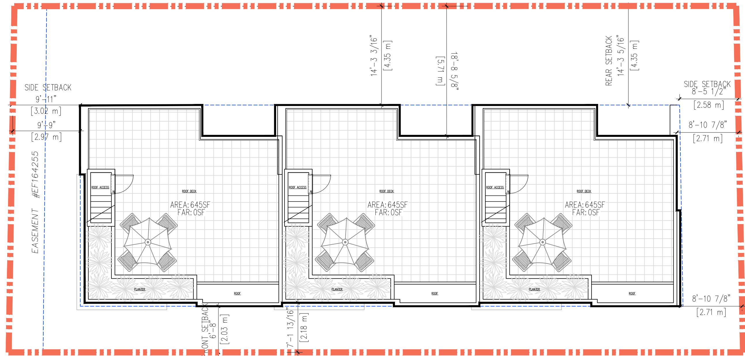
ROOF DECK PLAN
