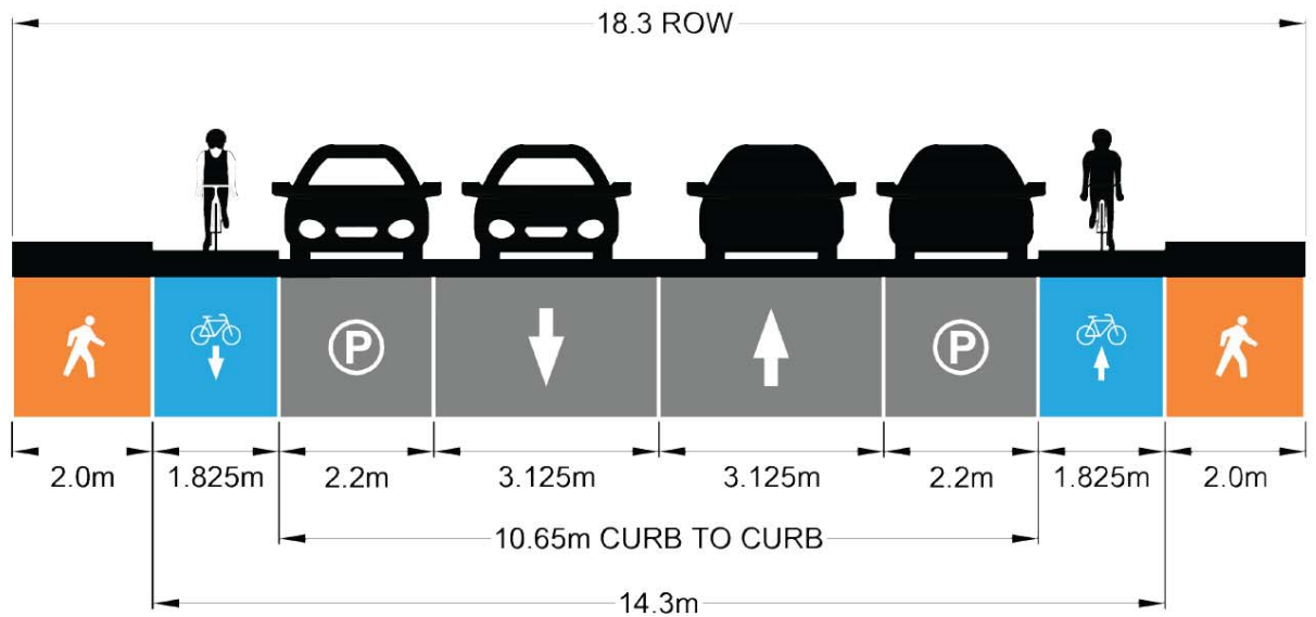
PROPOSED TYPICAL CROSS SECTION
