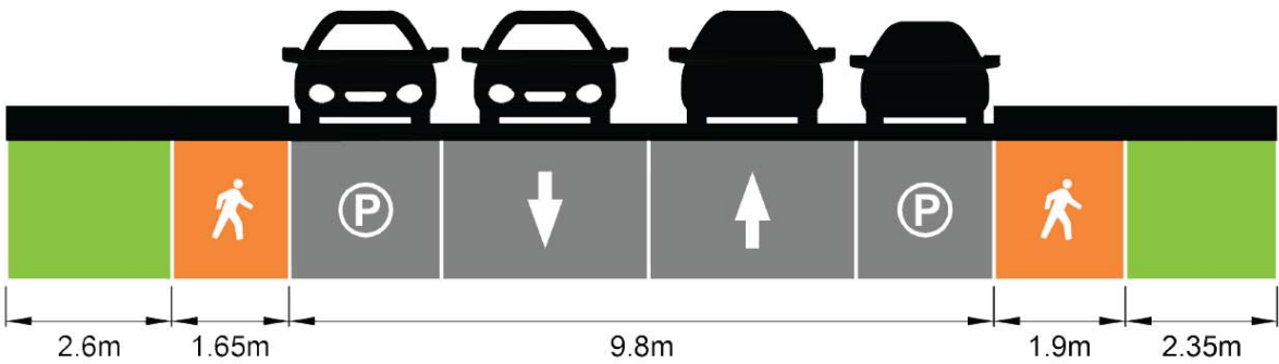
EXISTING TYPICAL CROSS SECTION (PARADISE ST TO HEAD ST)
