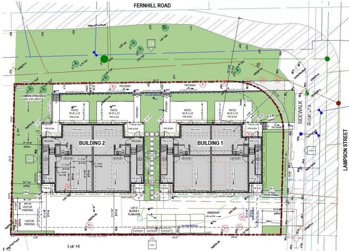
APPROVED SITEPLAN PER PLANNING & ENGINEERING REQUEST
