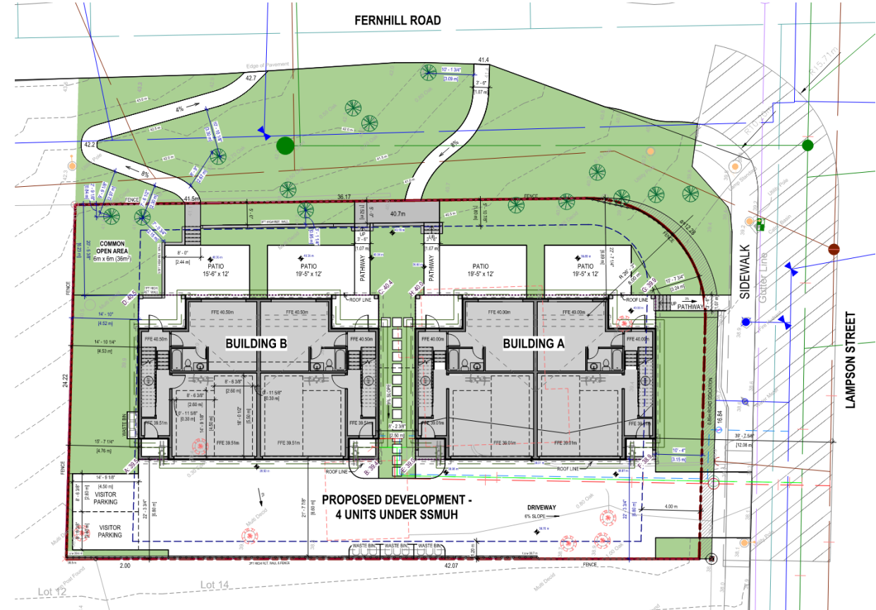
REQUESTED SITEPLAN
