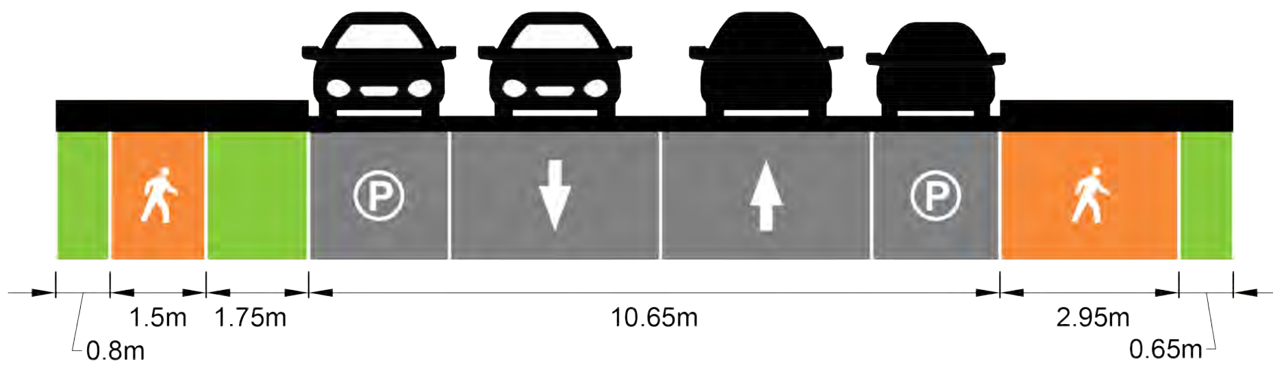
EXISTING TYPICAL CROSS SECTION (PARADISE ST TO HEAD ST)
