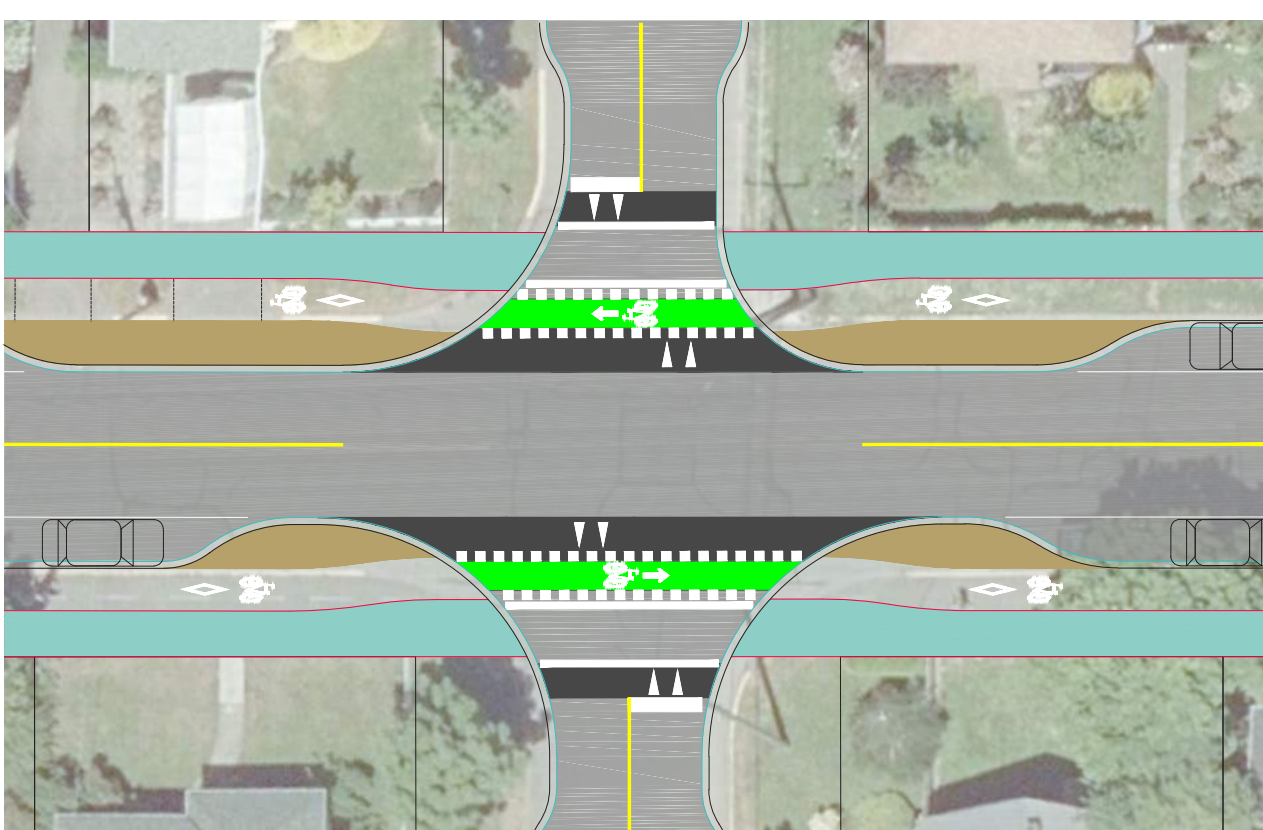
Protected Intersection Design
