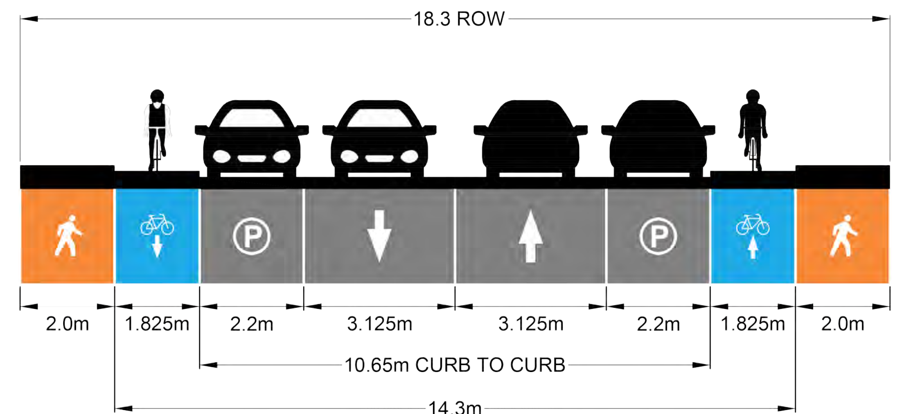
PROPOSED TYPICAL CROSS SECTION
